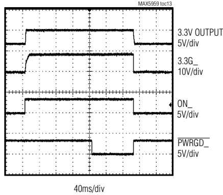
3.3V TURN-ON/OFF TIME
