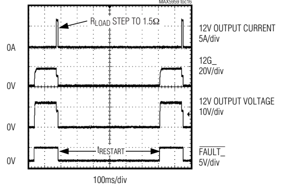
FAULT CONDITION ON 12V MAIN OUTPUT (AUTORESTART OPTION)
