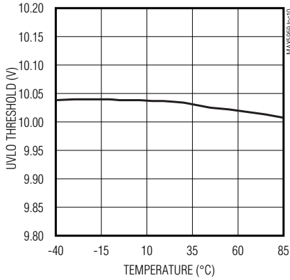
12V UNDERVOLTAGE LOCKOUT THRESHOLD vs. TEMPERATURE
