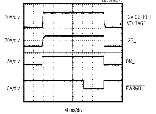
12V TURN-ON/OFF TIME
