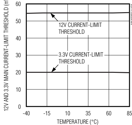
12V AND 3.3V MAIN CURRENT-LIMIT THRESHOLD VOLTAGE vs. TEMPERATURE
