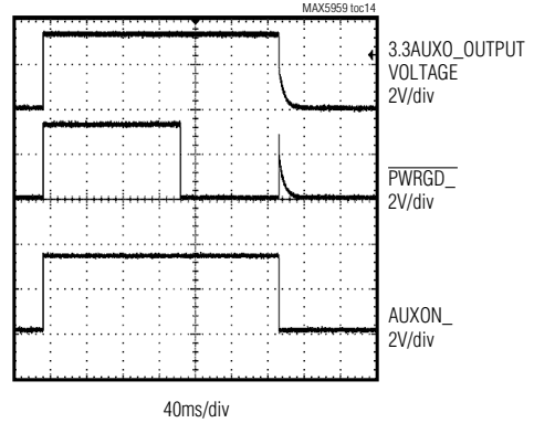
3.3V AUXILIARY TURN-ON/OFF TIME
